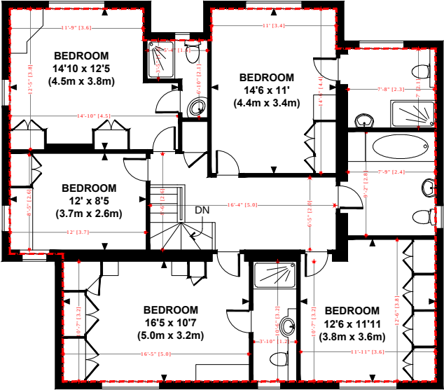
FIRST FLOOR area 162938 square in. (1131.52 square ft.)
